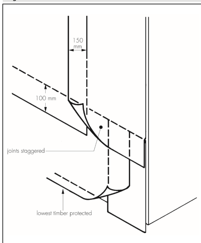
Figure 1 Membrane installation
